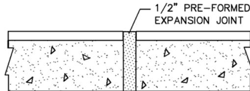
1/2" EXPANSION JOINT
